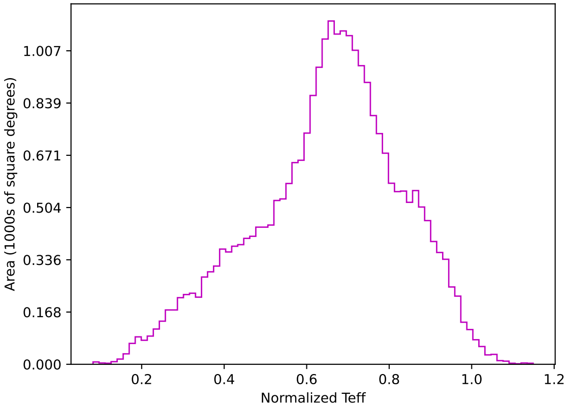
too_elab_r64_d2_ugrizy_v3.4_10yrs All sky z band: Normalized Teff
