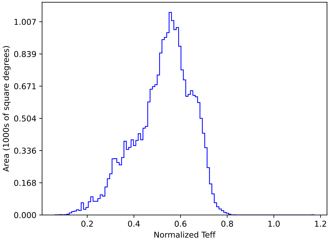
too_elab_r64_d2_ugrizy_v3.4_10yrs All sky y band: Normalized Teff
