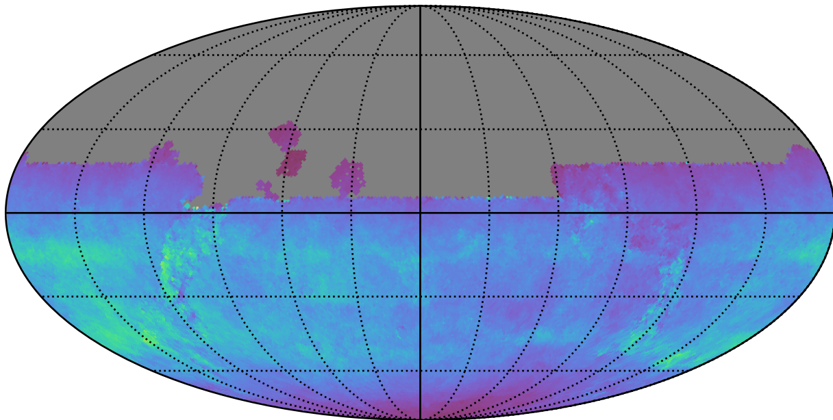
too_elab_r64_d2_ugrizy_v3.4_10yrs All sky u band: Normalized Teff
