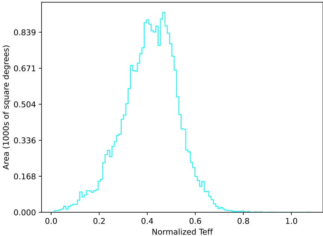
too_elab_r64_d2_ugrizy_v3.4_10yrs All sky u band: Normalized Teff
