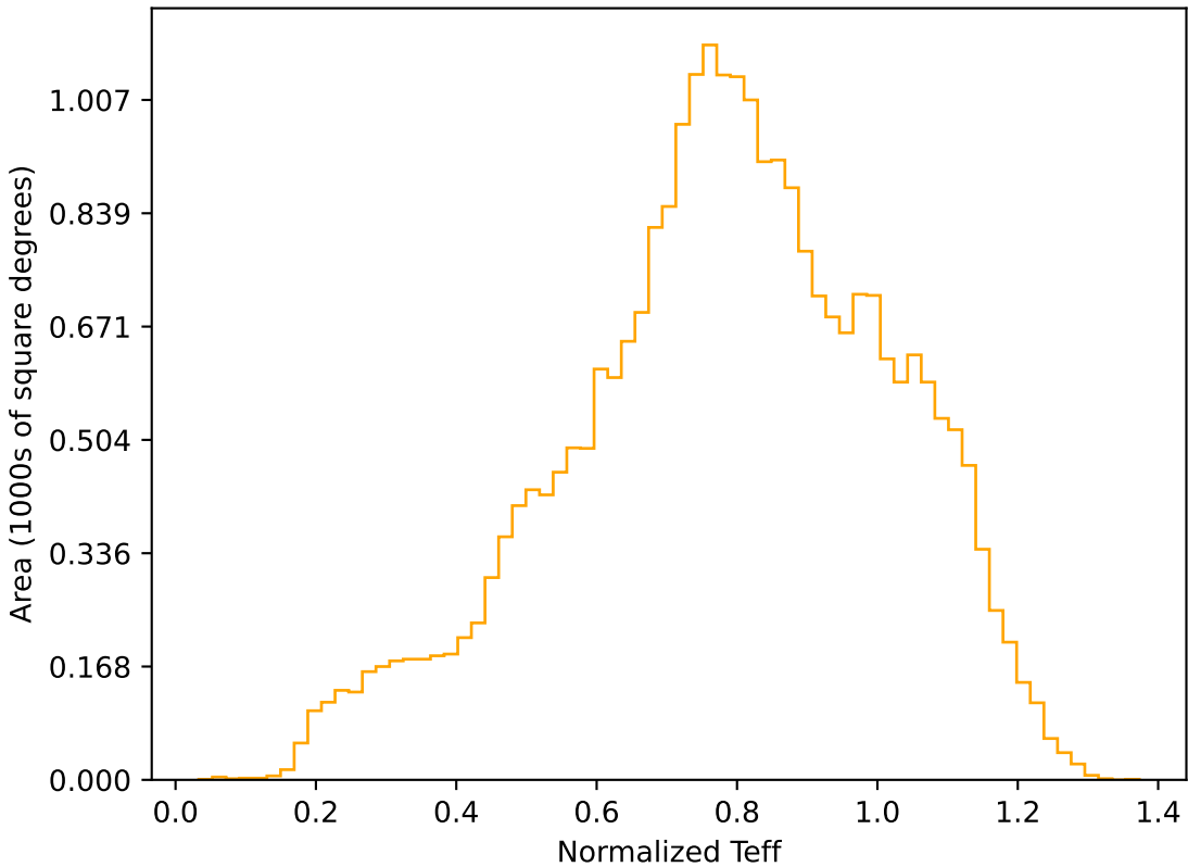
too_elab_r64_d2_ugrizy_v3.4_10yrs All sky r band: Normalized Teff
