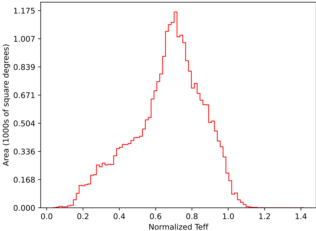
too_elab_r64_d2_ugrizyv3.4_10yrs All sky i band: Normalized Teff
