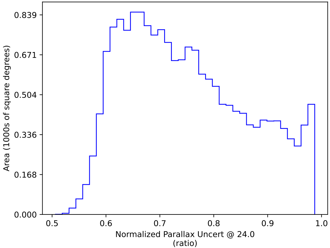
too_elab_r64_d2_ugrizy_v3.4_10yrs WFD: Normalized Parallax Uncert @ 24.0
