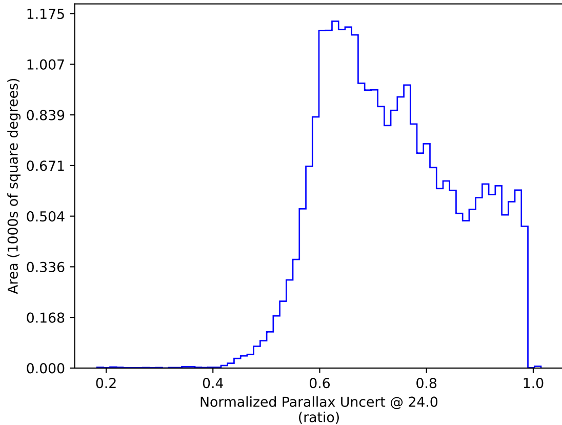
too_elab_r64_d2_ugrizy_v3.4_10yrs All sky: Normalized Parallax Uncert @ 24.0
