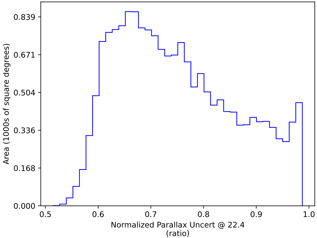
too_elab_r64_d2_ugrizy_v3.4_10yrs WFD: Normalized Parallax Uncert @ 22.4
