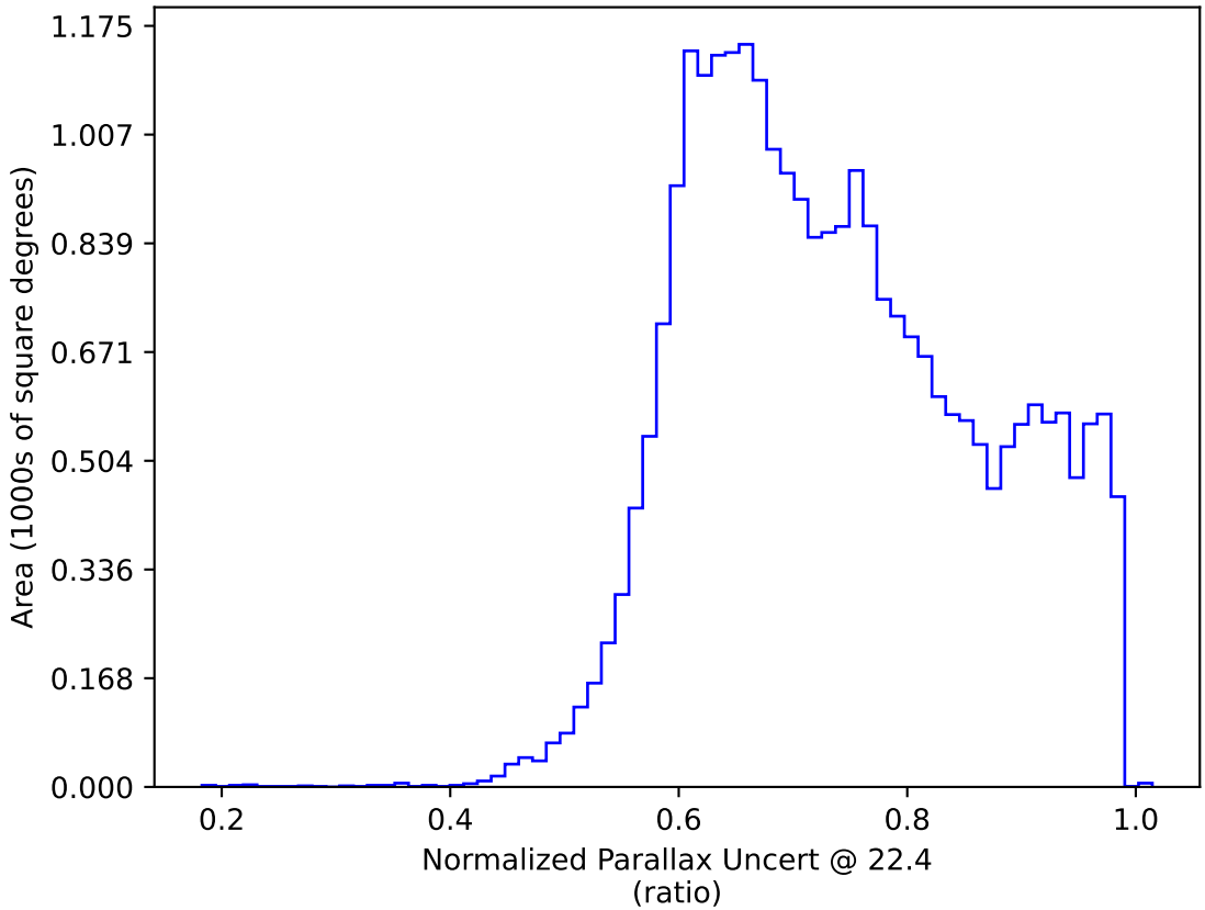
too_elab_r64_d2_ugrizy_v3.4_10yrs All sky: Normalized Parallax Uncert @ 22.4
