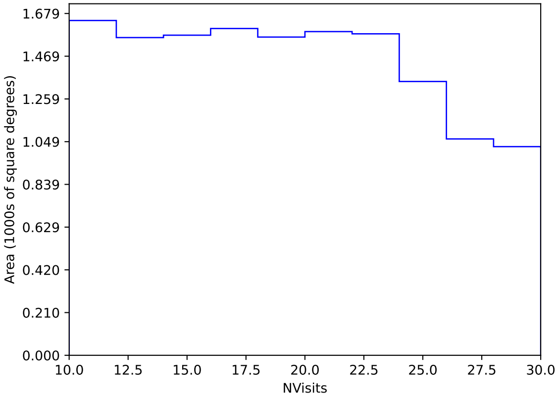
too_elab_r64_d2_ugrizy_v3.4_10yrs Yr 3-4 y band: NVisits
