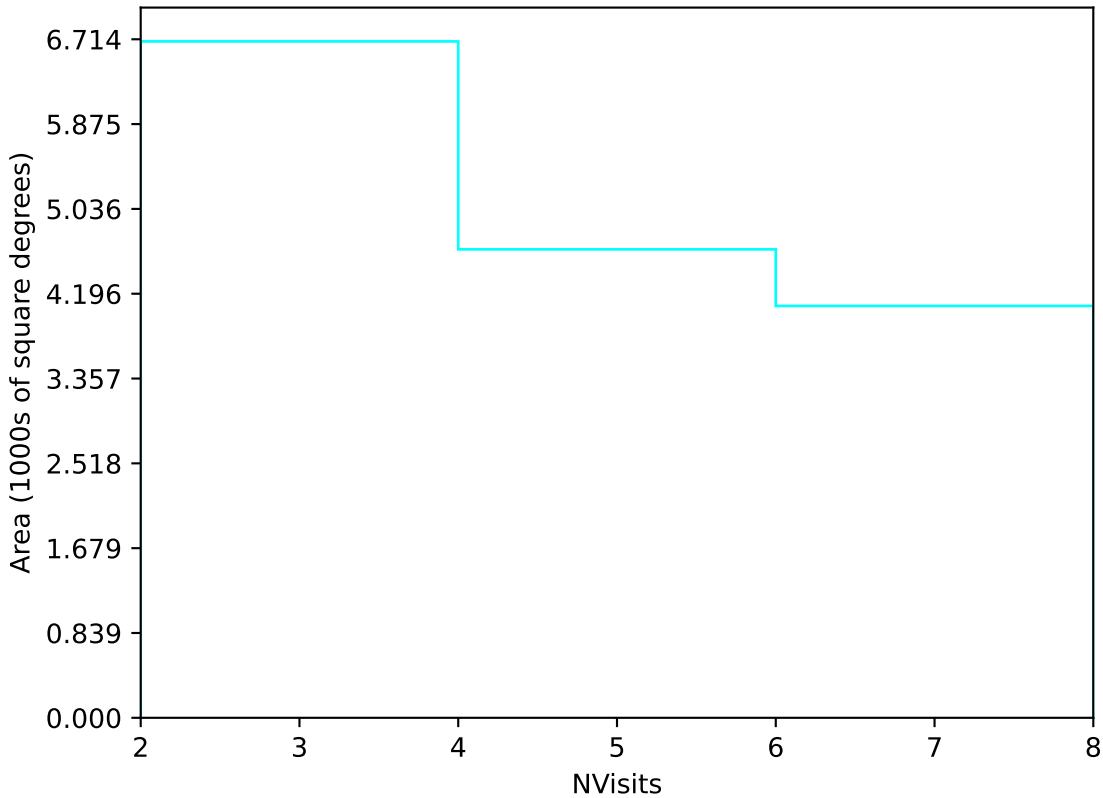
too_elab_r64_d2_ugrizy_v3.4_10yrs Yr 3-4 u band: NVisits
