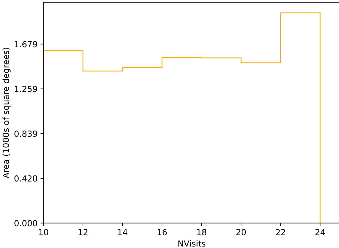
too_elab_r64_d2_ugrizy_v3.4_10yrs Yr 3-4 r band: NVisits
