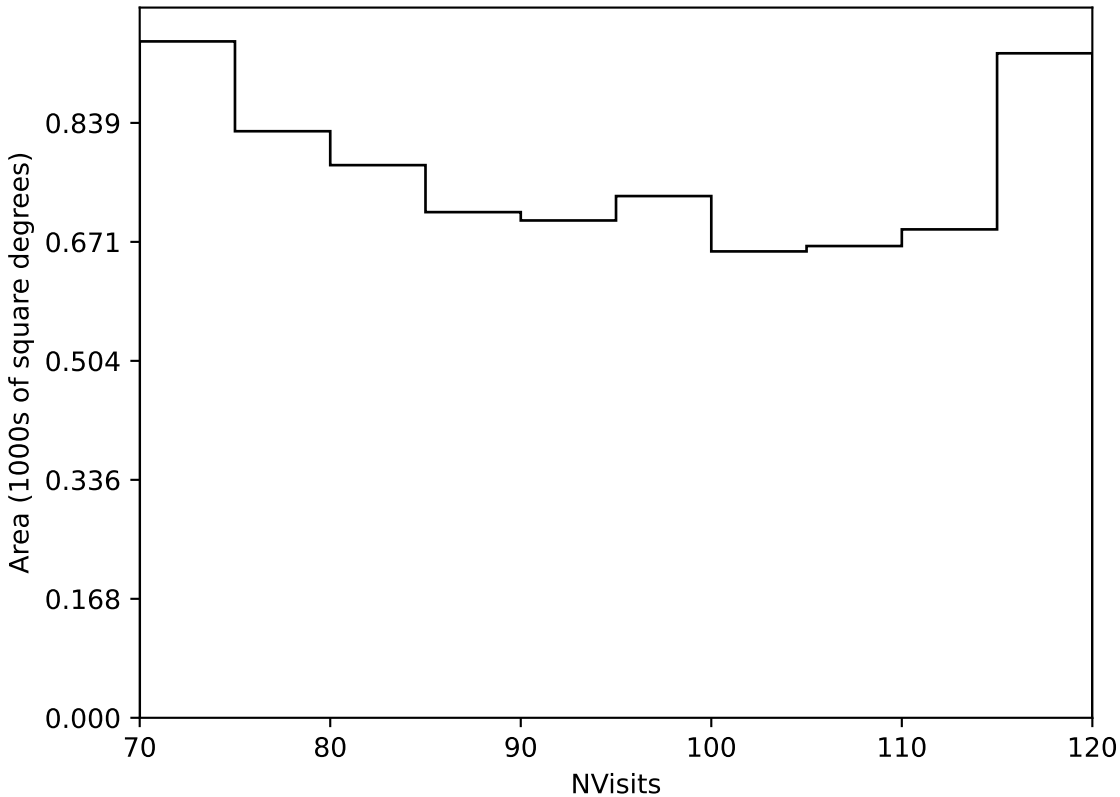
too_elab_r64_d2_ugrizy_v3.4_10yrs Yr 3-4 all bands: NVisits
