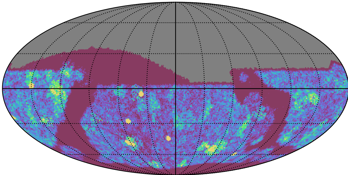
too_elab_r64_d2_ugrizy_v3.4_10yrs Yr 1 z band: NVisits
