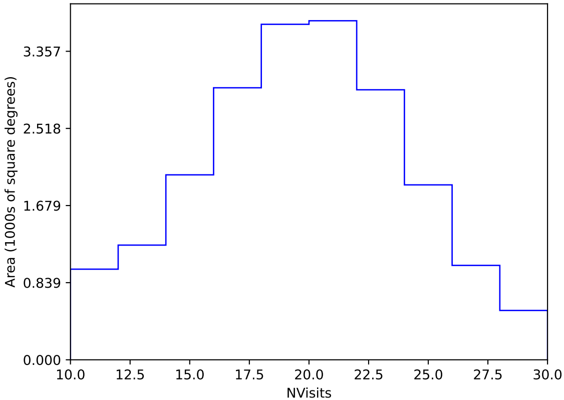
too_elab_r64_d2_ugrizy_v3.4_10yrs Yr 1 y band: NVisits
