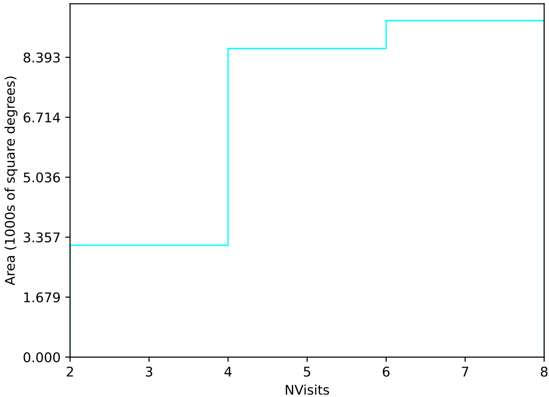
too_elab_r64_d2_ugrizy_v3.4_10yrs Yr 1 u band: NVisits
