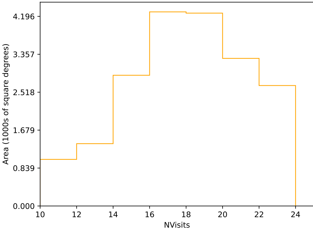
too_elab_r64_d2_ugrizy_v3.4_10yrs Yr 1 r band: NVisits
