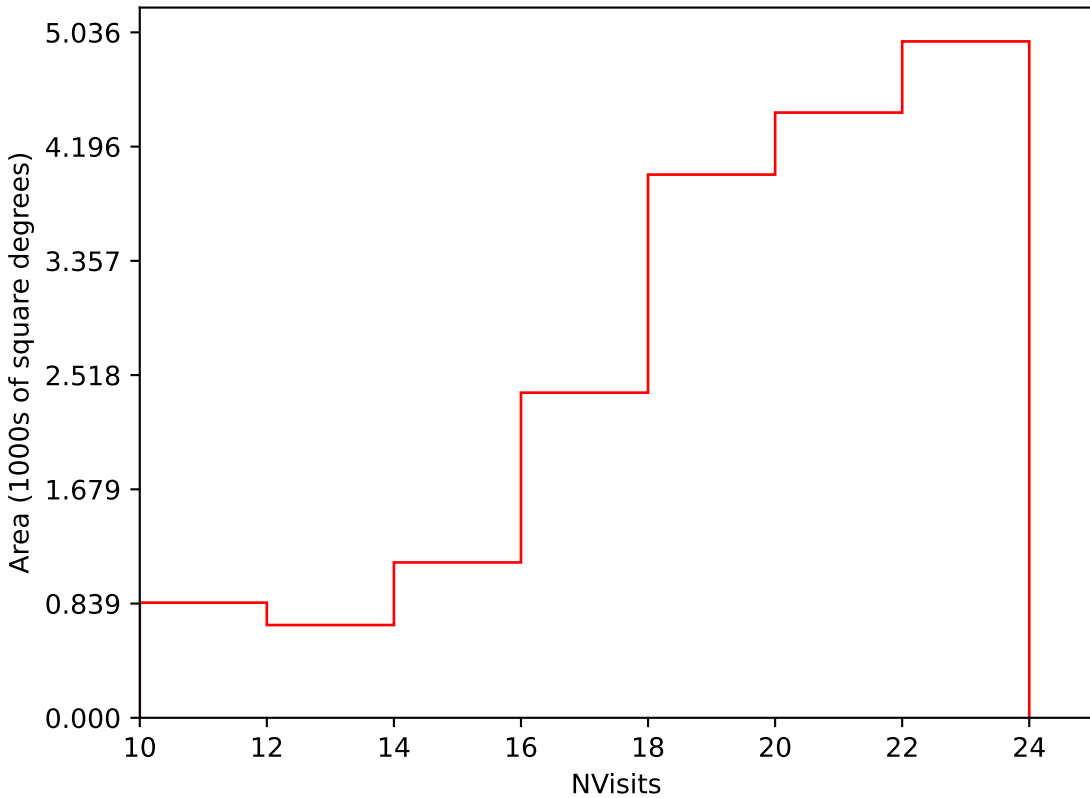
too_elab_r64_d2_ugrizy_v3.4_10yrs Yr 1 i band: NVisits
