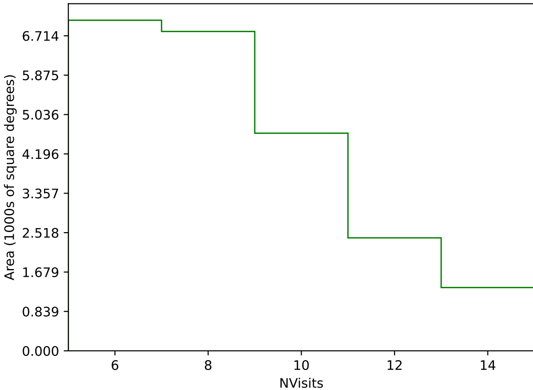
too_elab_r64_d2_ugrizy_v3.4_10yrs Yr 1 g band: NVisits
