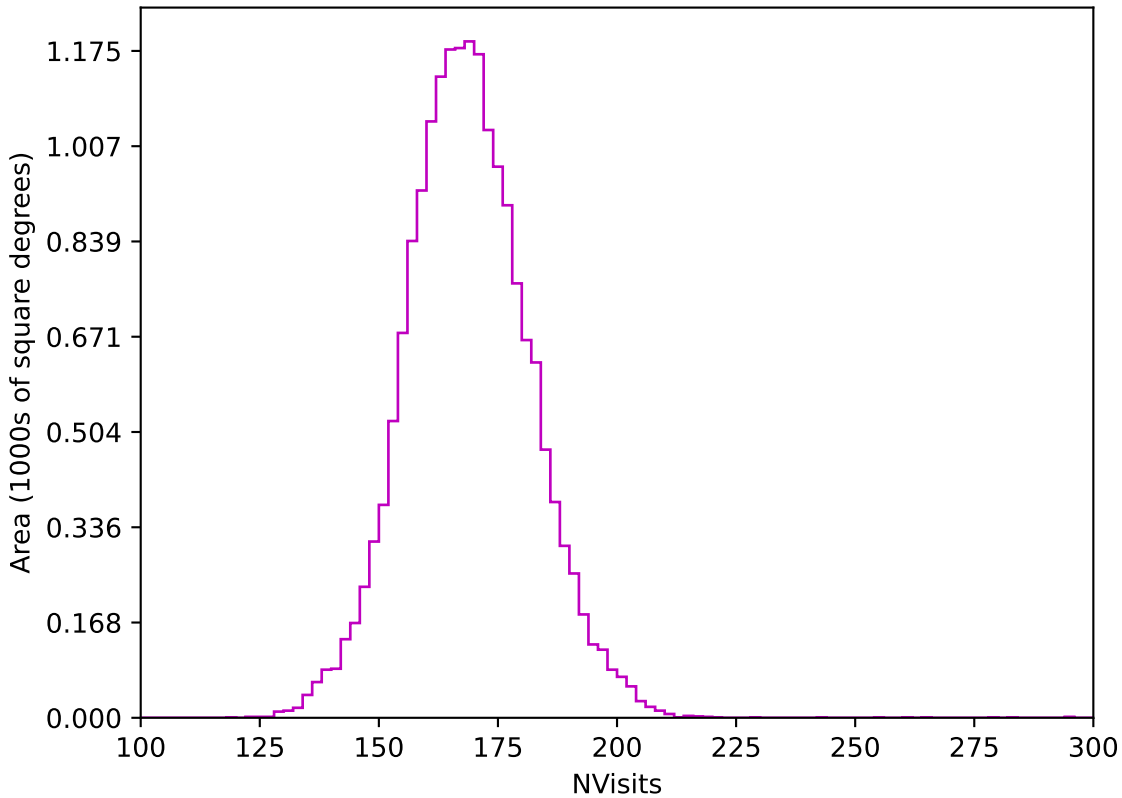
too_elab_r64_d2_ugrizy_v3.4_10yrs WFD z band: NVisits
