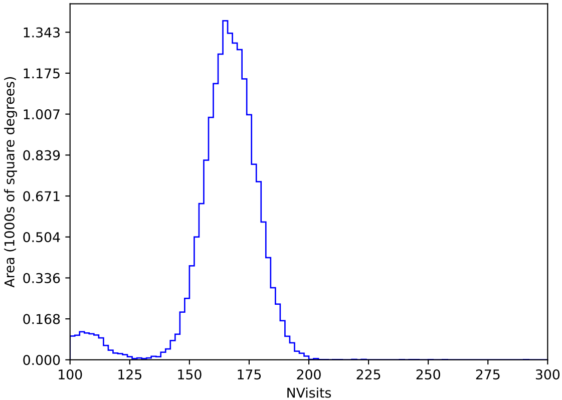
too_elab_r64_d2_ugrizy_v3.4_10yrs WFD y band: NVisits
