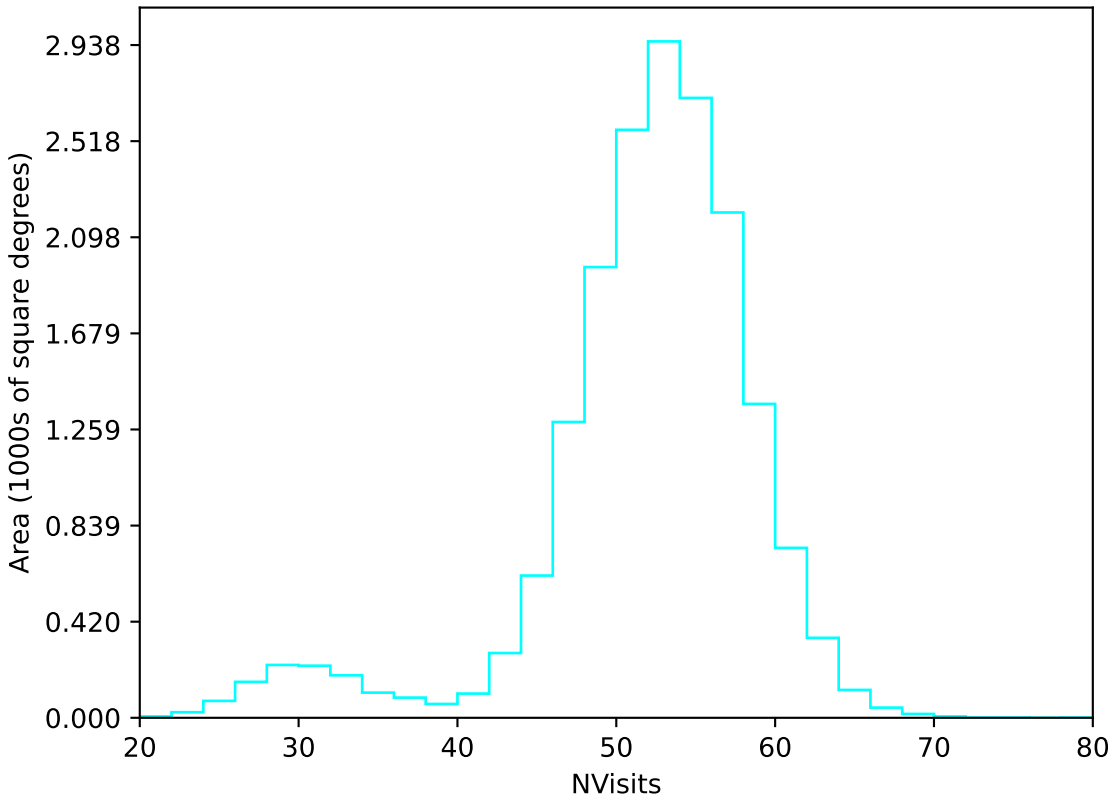
too_elab_r64_d2_ugrizy_v3.4_10yrs WFD u band: NVisits
