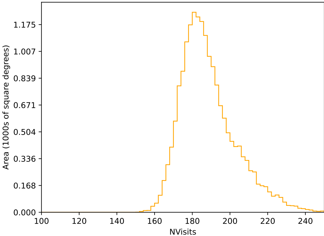
too_elab_r64_d2_ugrizy_v3.4_10yrs WFD r band: NVisits
