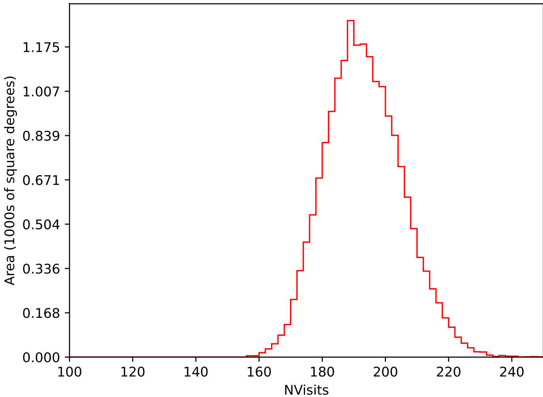
too_elab_r64_d2_ugrizy_v3.4_10yrs WFD i band: NVisits
