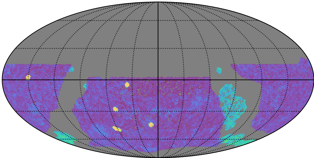
too_elab_r64_d2_ugrizy_v3.4_10yrs WFD g band: NVisits
