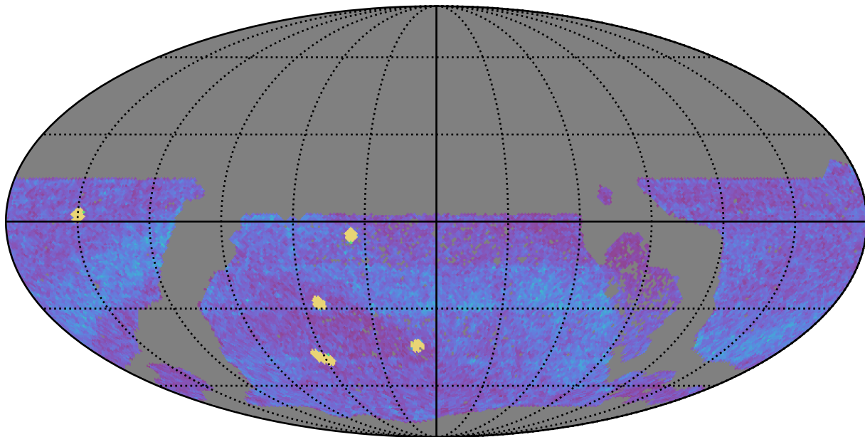
too_elab_r64_d2_ugrizy_v3.4_10yrs WFD all bands: NVisits
