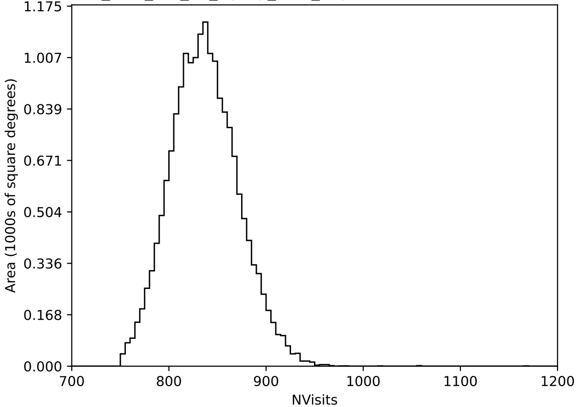
too_elab_r64_d2_ugrizy_v3.4_10yrs WFD all bands: NVisits
