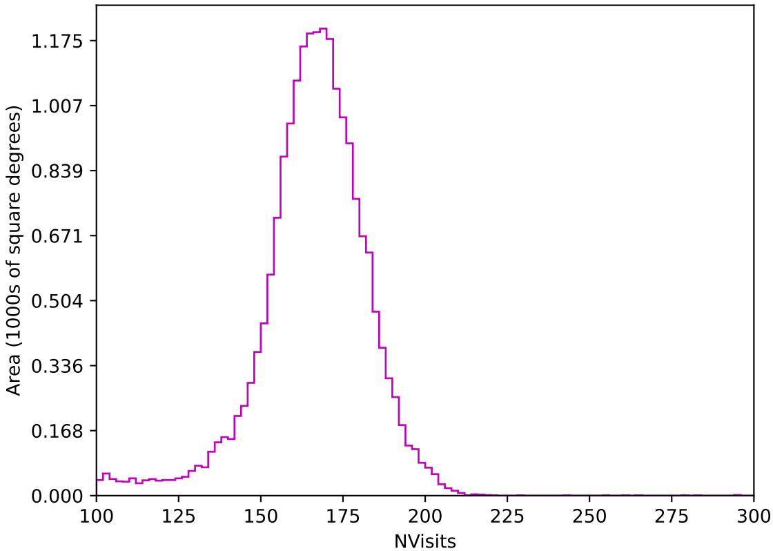
too_elab_r64_d2_ugrizy_v3.4_10yrs All sky z band: NVisits
