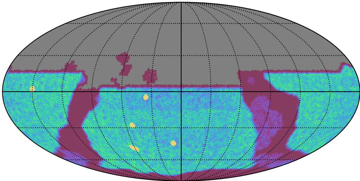
too_elab_r64_d2_ugrizy_v3.4_10yrs All sky u band: NVisits
