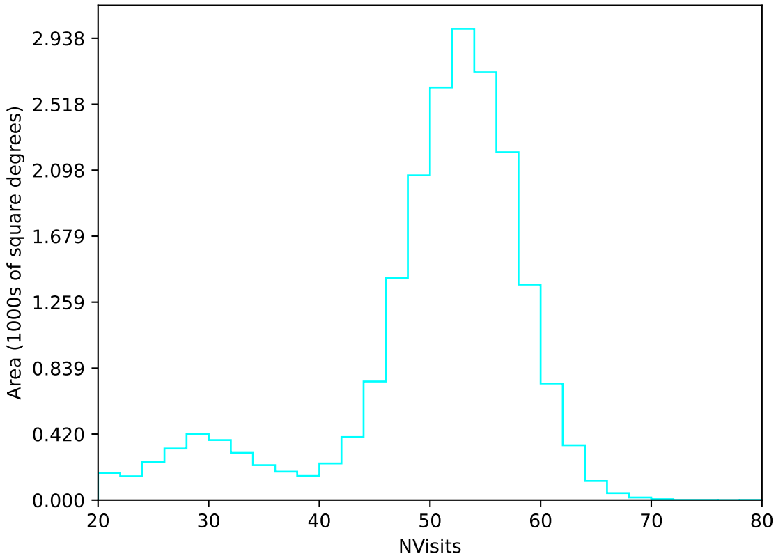
too_elab_r64_d2_ugrizy_v3.4_10yrs All sky u band: NVisits
