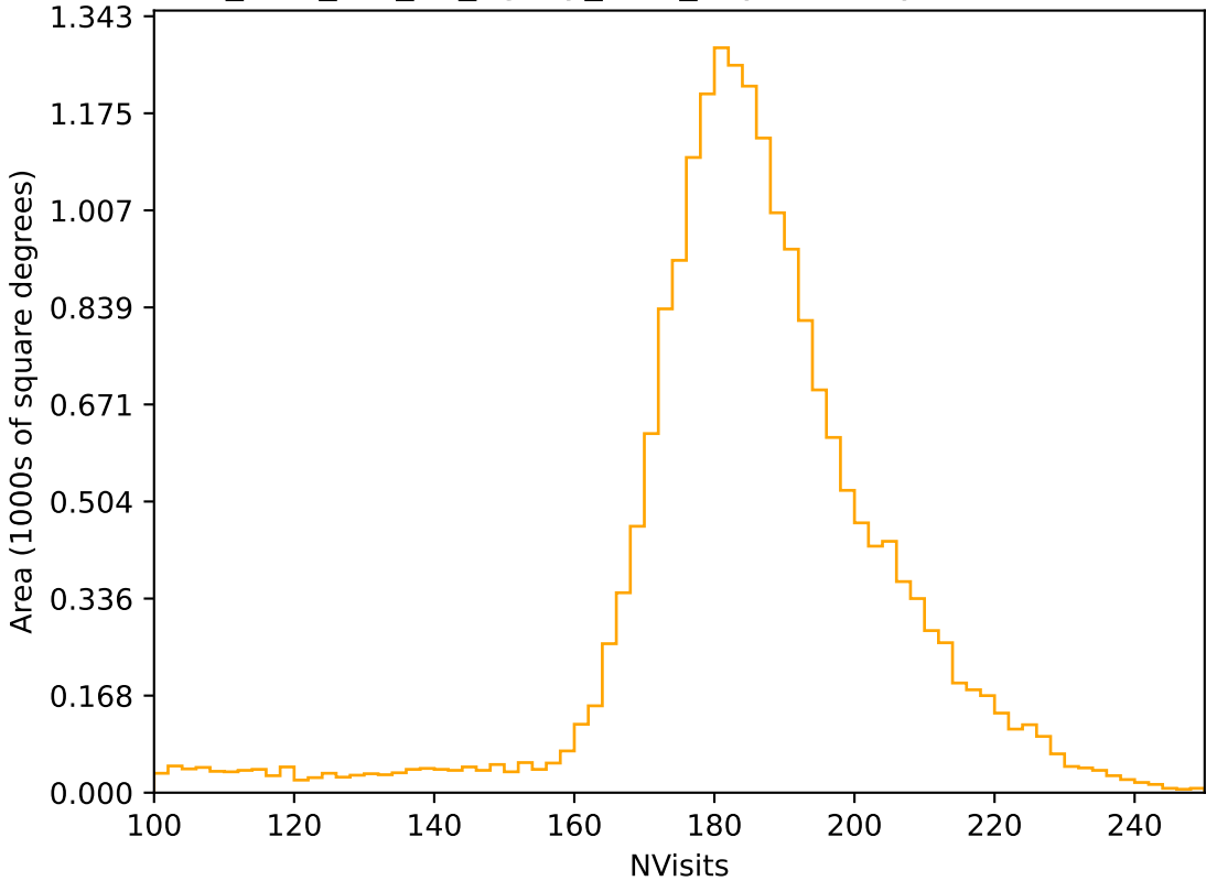
too_elab_r64_d2_ugrizy_v3.4_10yrs All sky r band: NVisits
