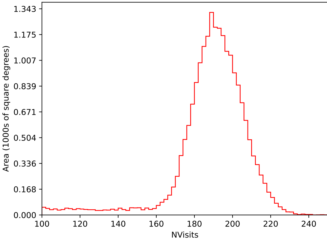
too_elab_r64_d2_ugrizy_v3.4_10yrs All sky i band: NVisits
