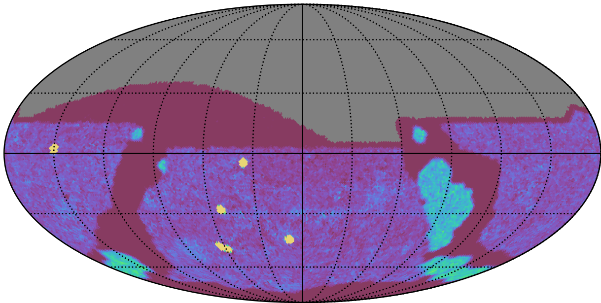
too_elab_r64_d2_ugrizy_v3.4_10yrs All sky g band: NVisits
