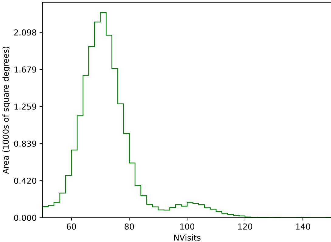
too_elab_r64_d2_ugrizy_v3.4_10yrs All sky g band: NVisits
