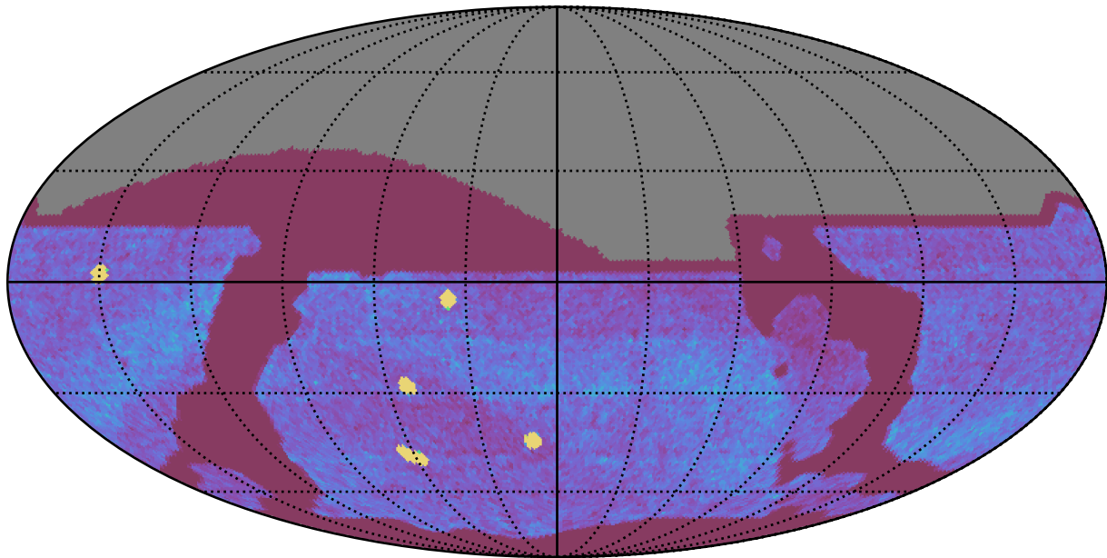
too_elab_r64_d2_ugrizy_v3.4_10yrs All sky all bands: NVisits
