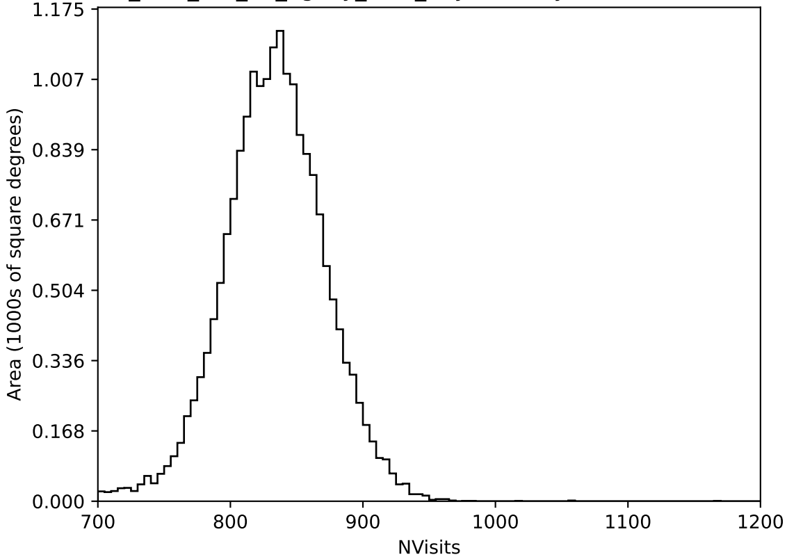
too_elab_r64_d2_ugrizy_v3.4_10yrs All sky all bands: NVisits
