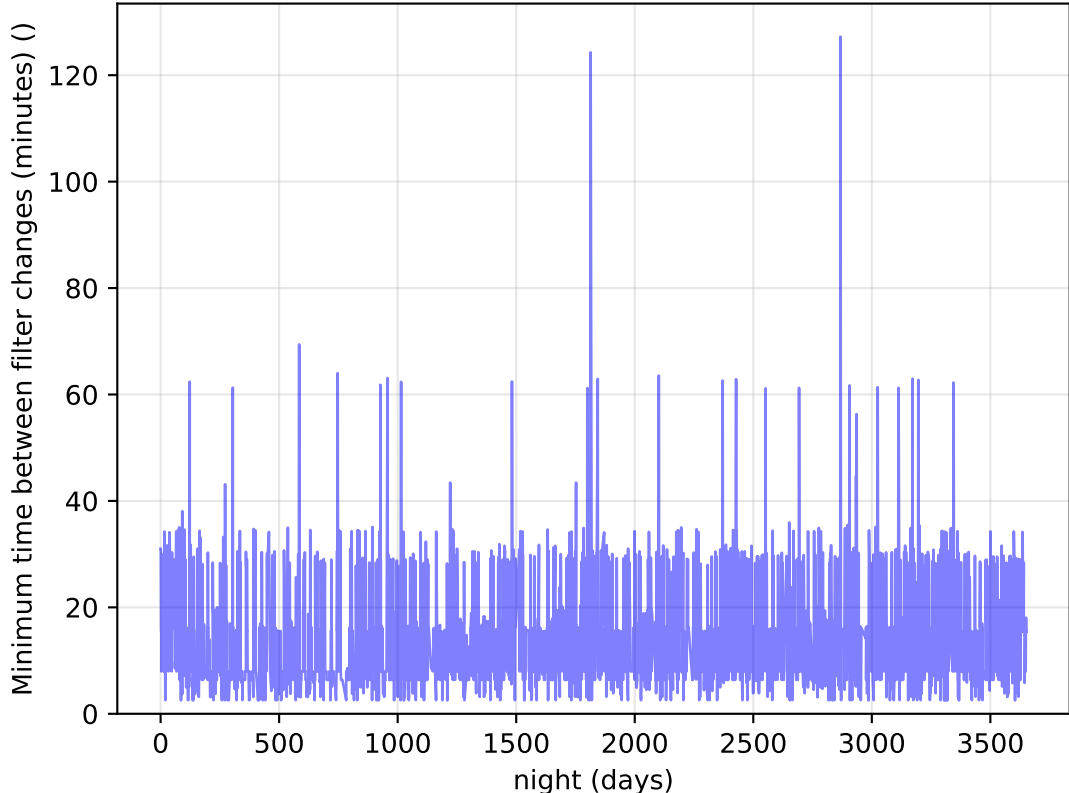
too_elab_r64_d2_ugrizy_v3.4_10yrs Per Night: Minimum time between filter changes (minutes)
