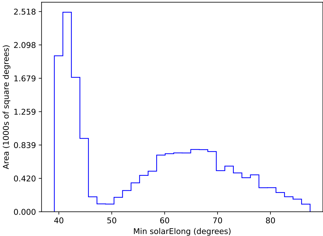
too_elab_r64_d2_ugrizy_v3.4_10yrs WFD r band: Min solarElong
