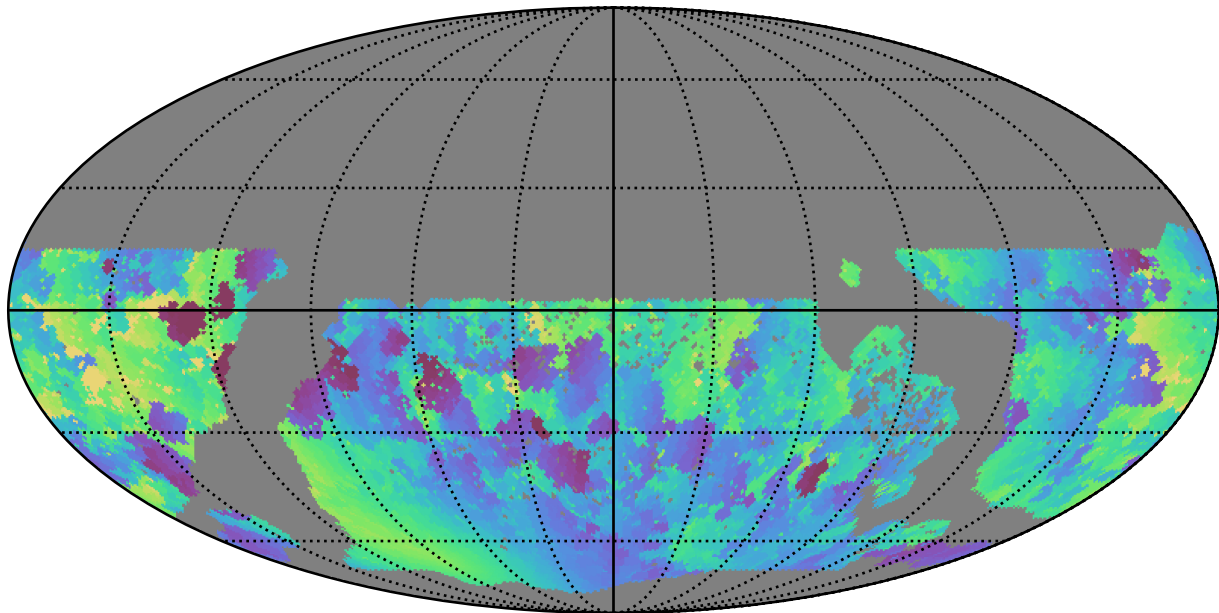
too_elab_r64_d2_ugrizy_v3.4_10yrs WFD g band: Min solarElong
