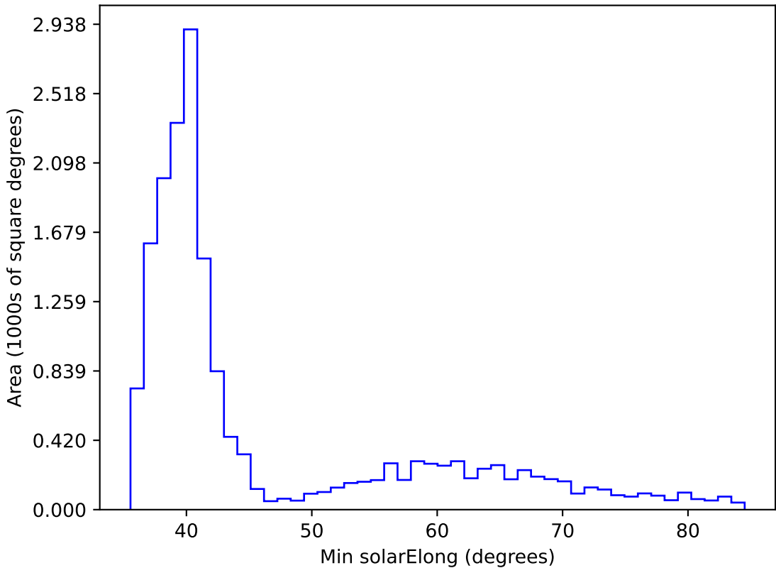
too_elab_r64_d2_ugrizy_v3.4_10yrs WFD all bands: Min solarElong
