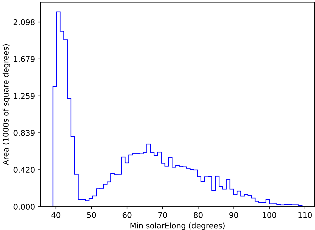
too_elab_r64_d2_ugrizy_v3.4_10yrs All sky r band: Min solarElong
