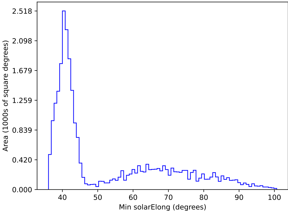
too_elab_r64_d2_ugrizy_v3.4_10yrs All sky i band: Min solarElong
