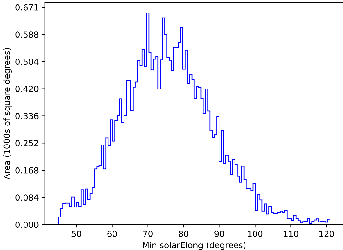
too_elab_r64_d2_ugrizy_v3.4_10yrs All sky g band: Min solarElong
