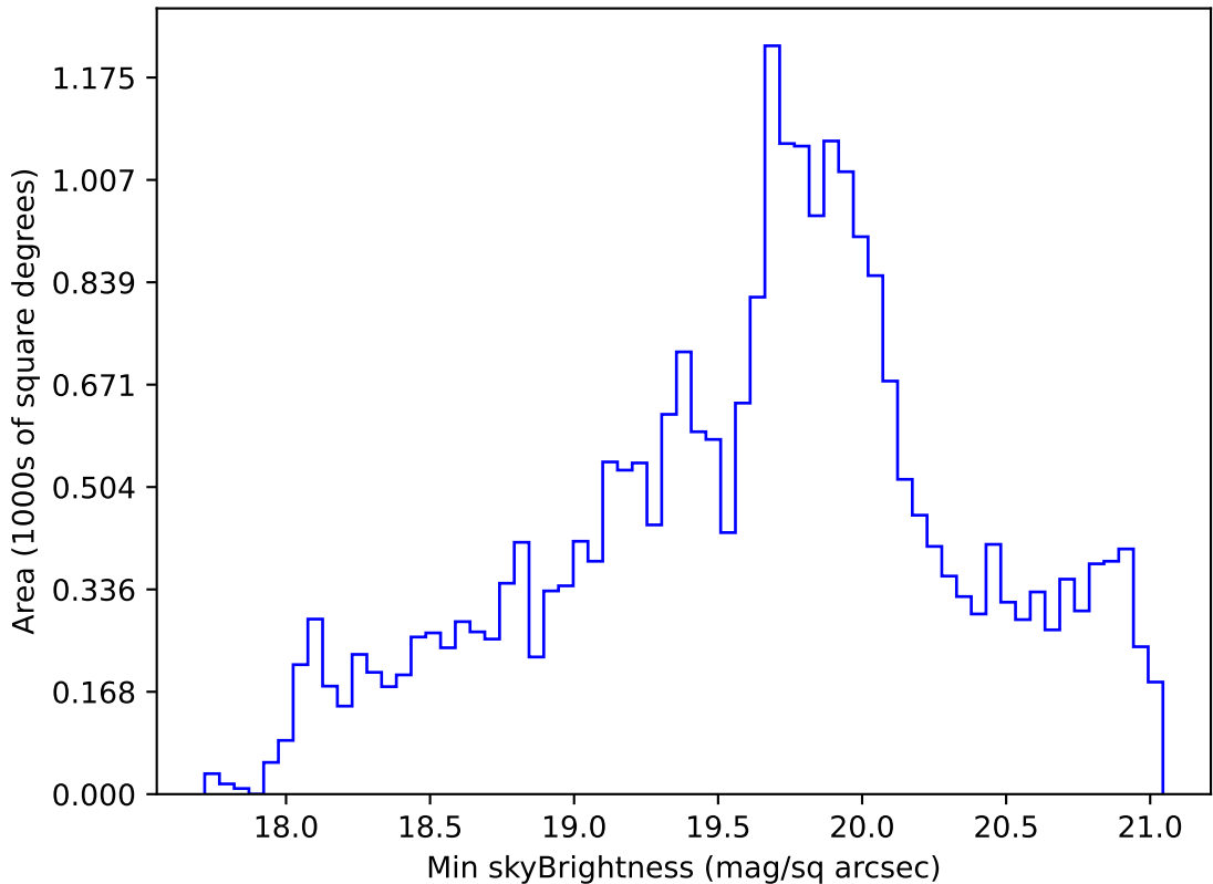
too_elab_r64_d2_ugrizy_v3.4_10yrs Yr 1 r band: Min skyBrightness
