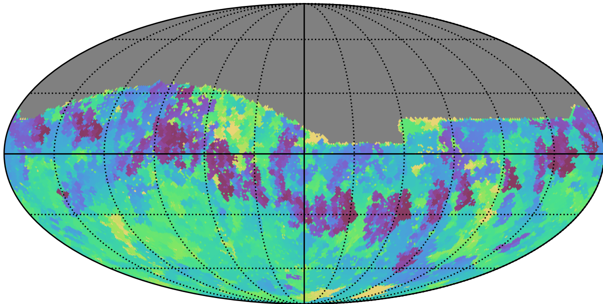
too_elab_r64_d2_ugrizy_v3.4_10yrs Yr 1 i band: Min skyBrightness
