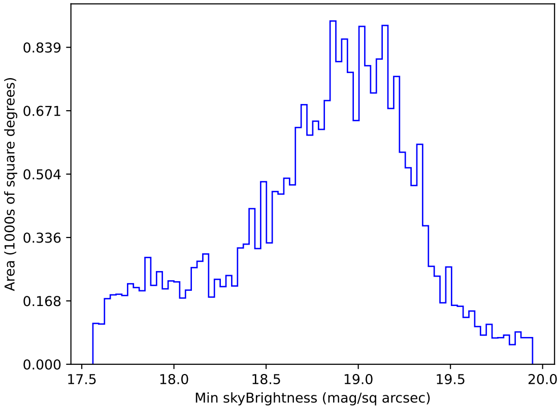
too_elab_r64_d2_ugrizy_v3.4_10yrs Yr 1 i band: Min skyBrightness
