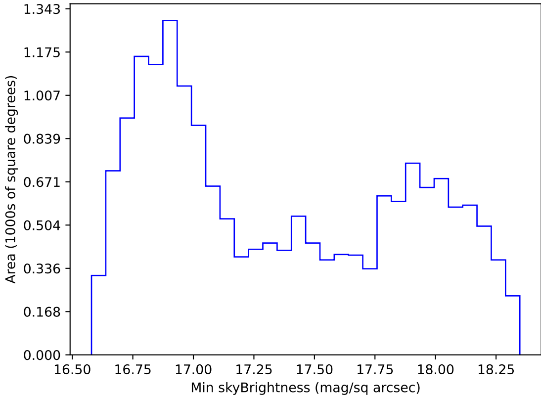
too_elab_r64_d2_ugrizy_v3.4_10yrs WFD z band: Min skyBrightness
