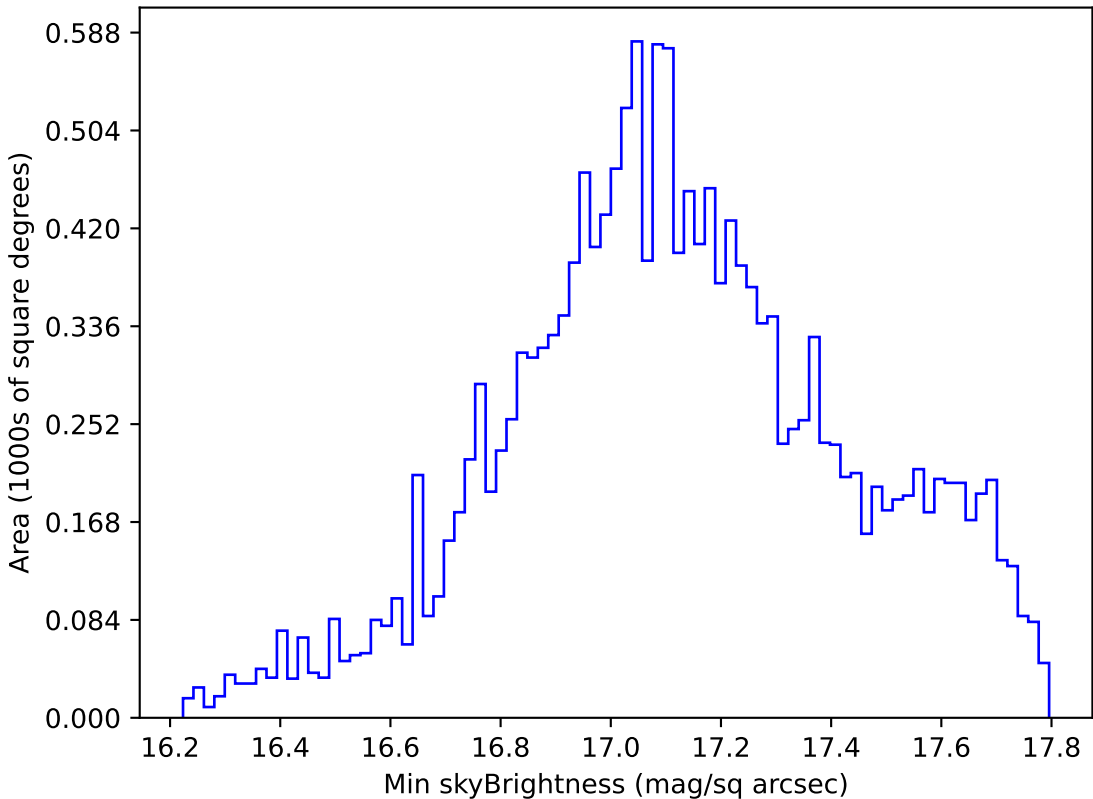
too_elab_r64_d2_ugrizy_v3.4_10yrs WFD y band: Min skyBrightness
