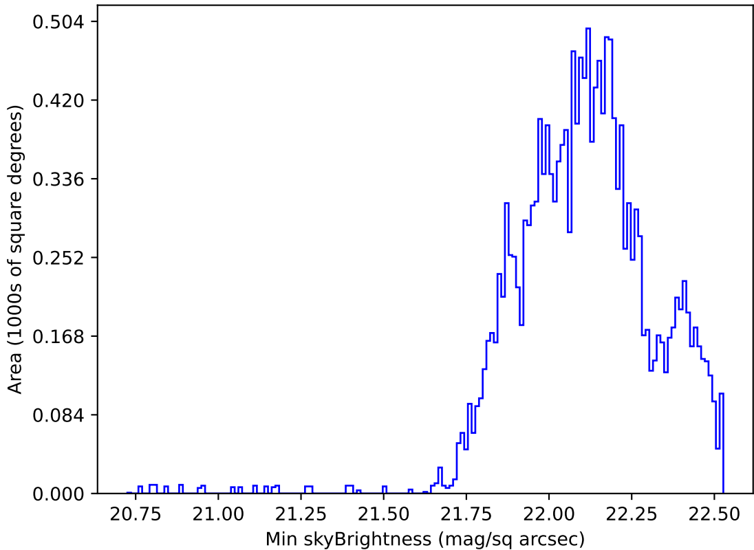
too_elab_r64_d2_ugrizy_v3.4_10yrs WFD u band: Min skyBrightness
